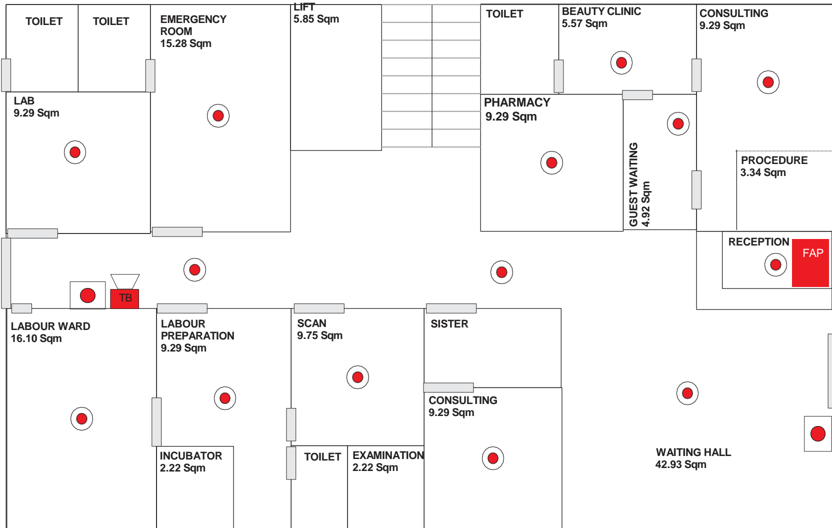
GROUND FLOOR
